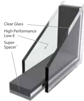
ComforTech™ DLE ComforTech™ DLE-UV ●●●○○○○○○○ R-Value of 3
