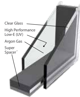
ComforTech™ DLA-UV ●●●●○○○○○○○ R-Value of 4
