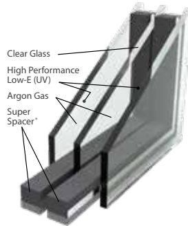
ComforTech™ TLA-UV ●●●●●●●○○○ R-Value of 6
